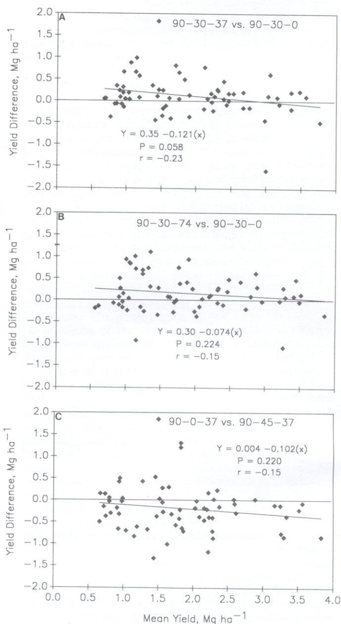
Fig. 7. (a-c). Relative stability of treatment pairs, Exp. #222, Stillwater, Ok, 1969-1987.
